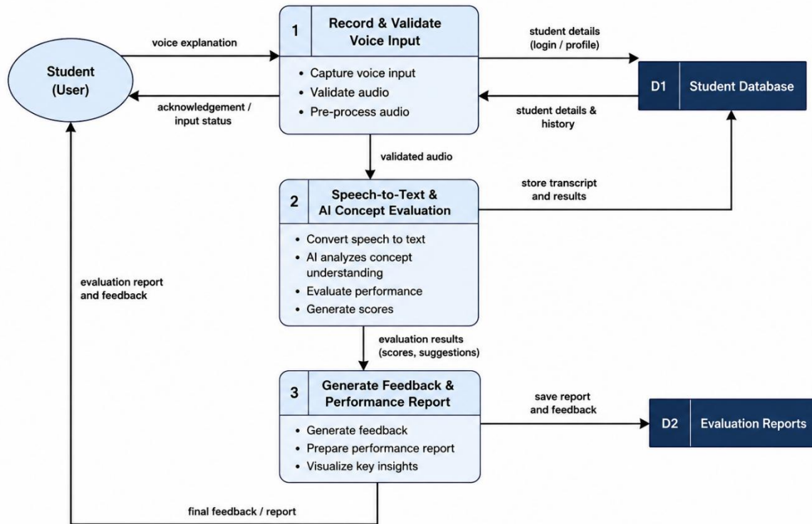
Data Flow Diagram (DFD) – Voice-Based Concept Understanding Analyzer
